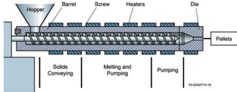
Figure 9 Extruder for Biomass or polymer processing (Tumuluru, 2011)
