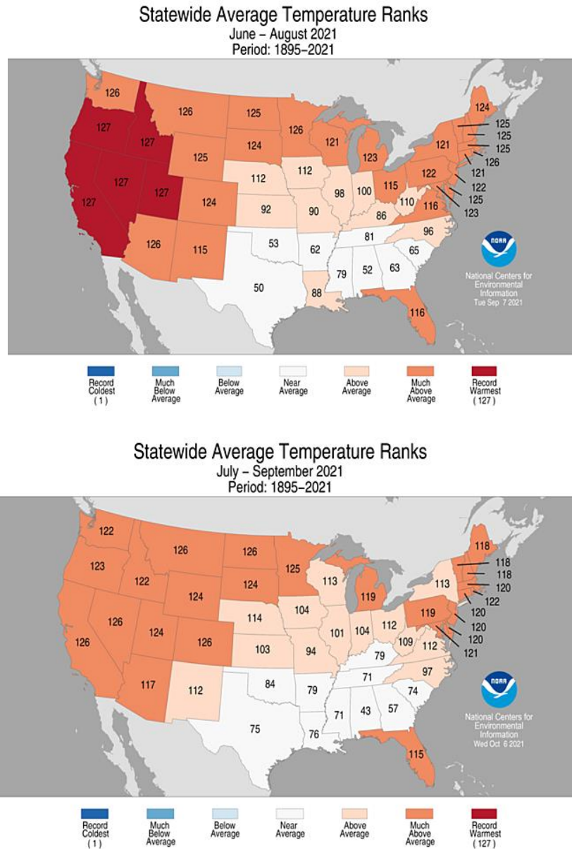
Figure 11: NCDC Statewide Average Temperature Ranks for June – August 2021.
