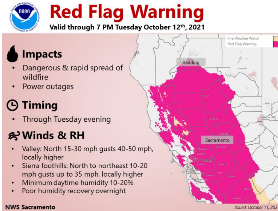
Figure 15: NWS Red Flag Warning Coverage from the Sacramento Weather Office
