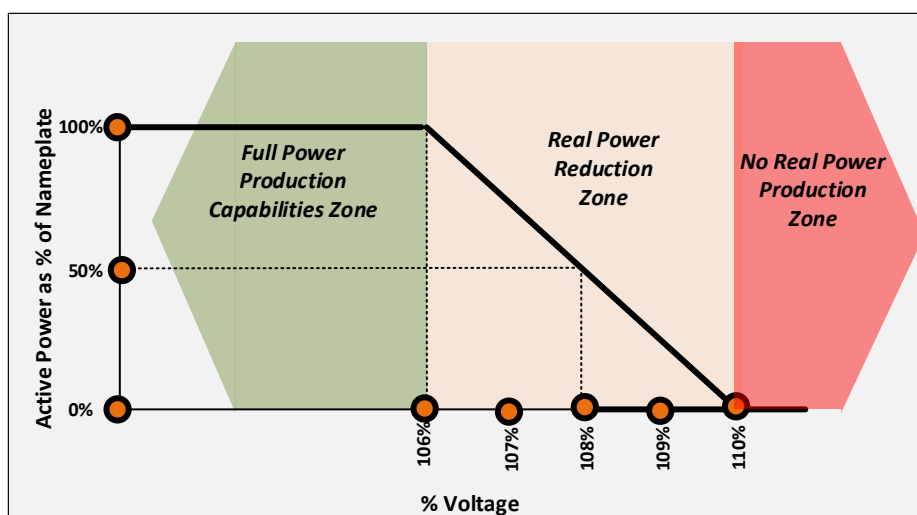
Figure Hh-3: Volt-Watt Requirements
